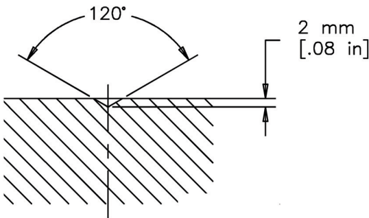
Figure 2—Dimple Dimensions
