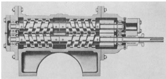
FIGURE 12 Double-end internal gear design. (Flowservice Corporation)
