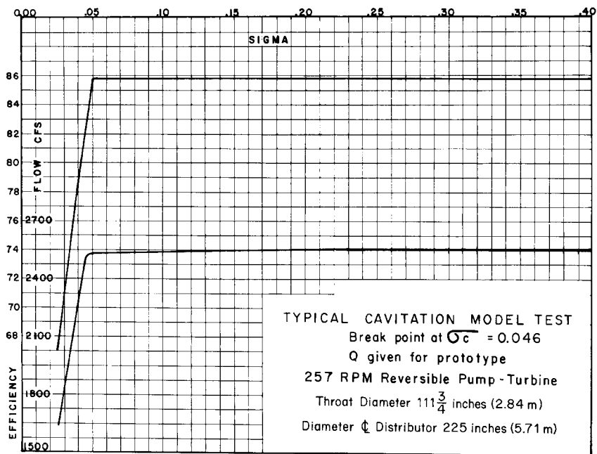
FIGURE 5 Typical cavitation model test (1 ft³/s = 0.0283 m³/s) (Voith Siemens Hydro)
