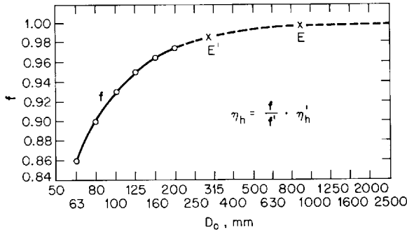
FIGURE 58 The f function for the Rütshi formula (to obtain D_o in inches, multiply by 0.03937) (References 13 and 62)
