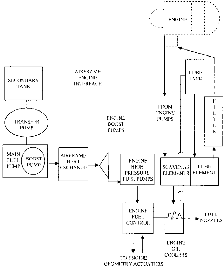
FIGURE 1 Basic schematic of fuel system
