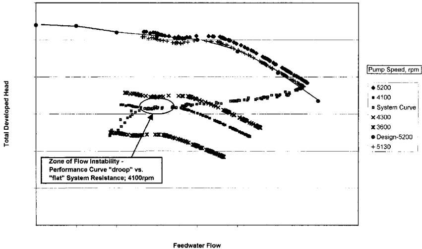
FIGURE 14 Performance characteristic—28,000 hp boiler feed pump ( N_s = 1700 ) (Universal specific speed \Omega_s = N_s/2733 \cdot N_q (in rpm, m^3/s , m) = N_s/51.65 )
