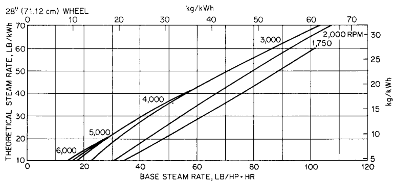
FIGURE 7 Base steam rates (Elliott)
