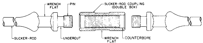
FIGURE 4 A typical sucker rod joint (API)
