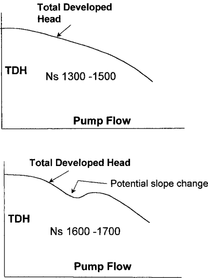
FIGURE 13 Pump performance curve characteristic—specific speed versus stability (Universal specific speed \Omega_s = N_s/2733 \cdot N_q (in rpm, m^3/s , m) = N_s/51.65 )
