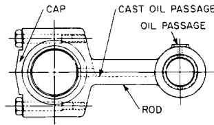
FIGURE 19 The connecting rod (Flowserve Corporation)
