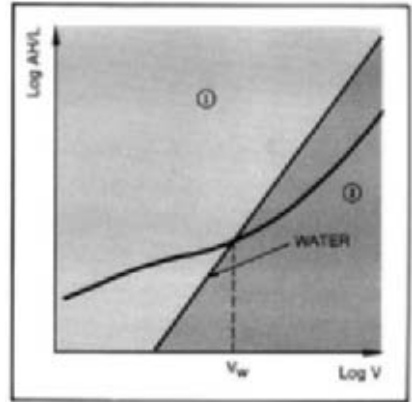
FIGURE 10 Friction loss curves for mechanical pulp, shaded to show individual regions. (Courtesy ITT / Goulds Pumps, Inc.)
