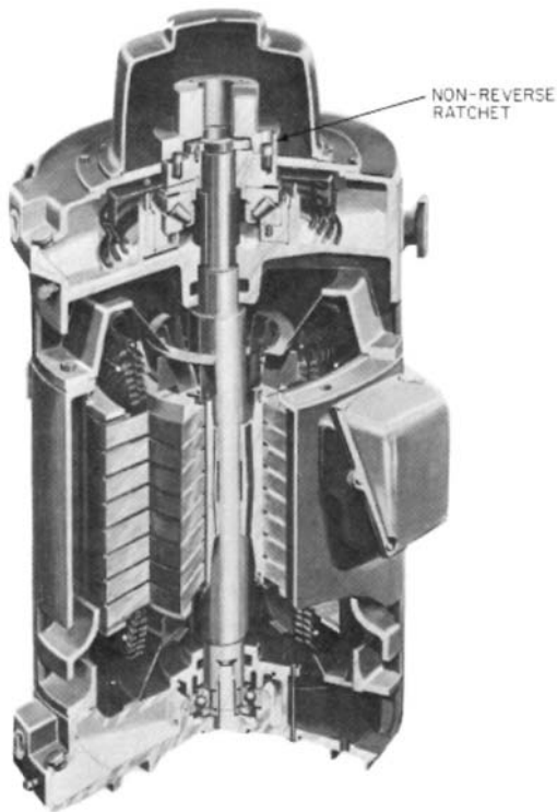
FIGURE 18 Section of vertical hollow shaft motor showing nonreverse ratchet. Spring-loaded pins ride on ratchet plate in one direction only (General Electric).
