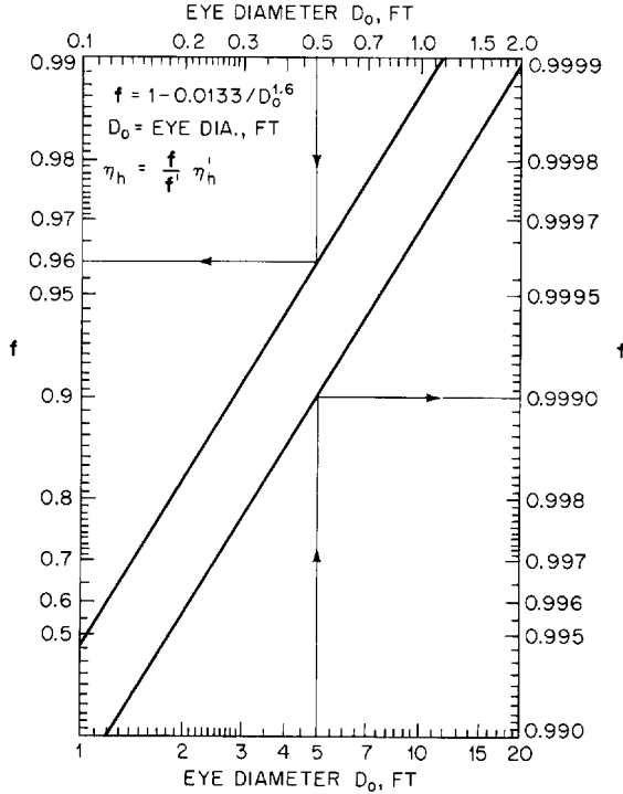
FIGURE 59 Chart for the solution of the Rütshi formula (to obtain D_o in meters, multiply by 0.3048) (Reference 62)
